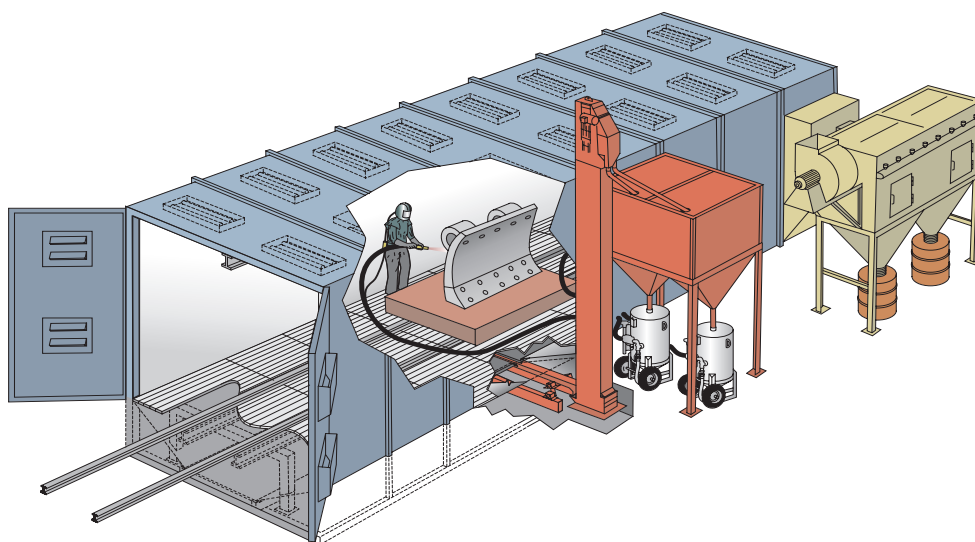
BLAST ROOM WITH RAIL TRACKS INCREASES PRODUCTIVITY FOR MATERIAL HANDLING
