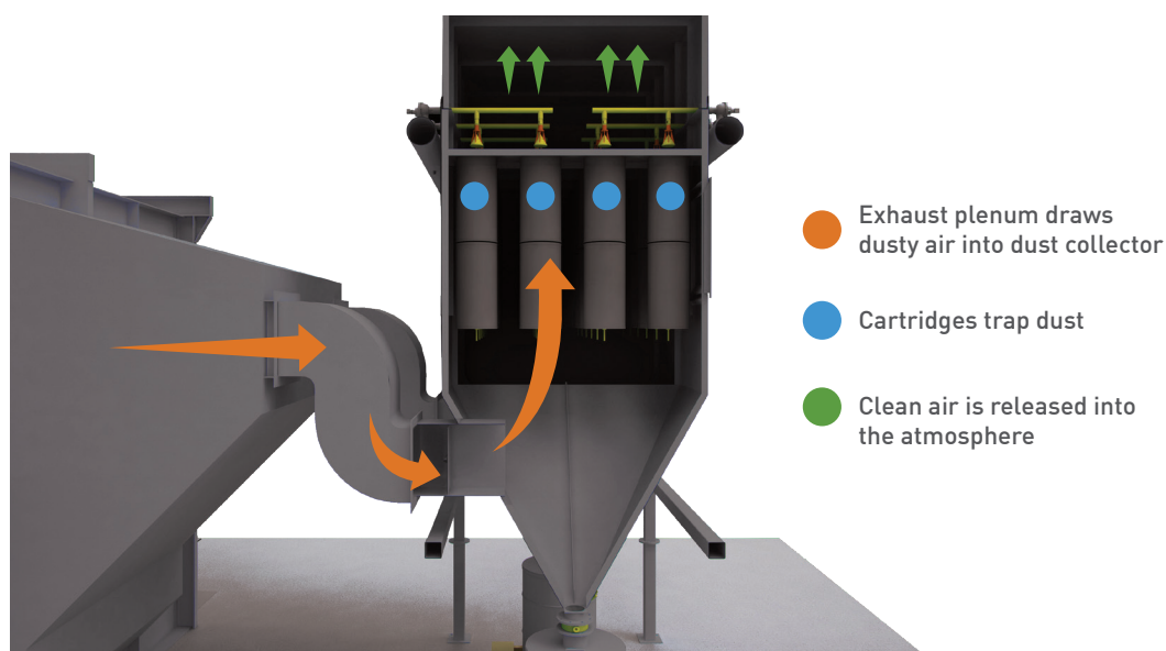
DIAGRAM SHOWS THE PATH OF THE AIRFLOW
